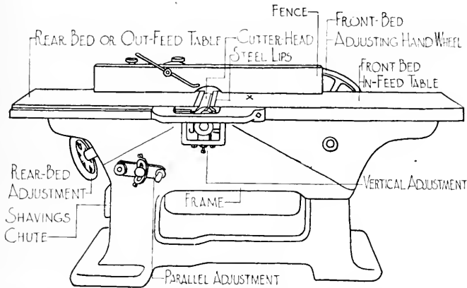
FIG. 135. HAND PLANER OR JOINTER.
